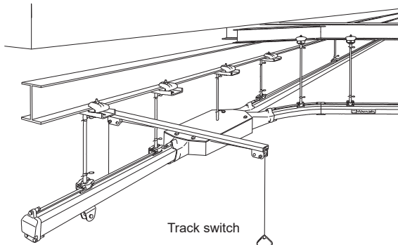
Suspension monorail
