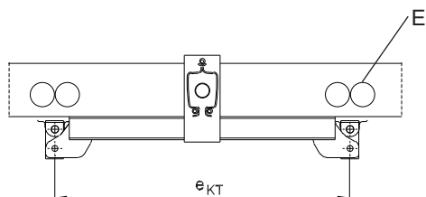
KBK II-L/II crane end carriage, raised, Single-girder suspension crane (EHK)
