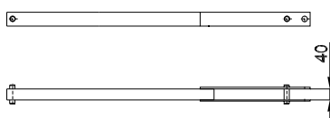
Spacer bar with one open end
