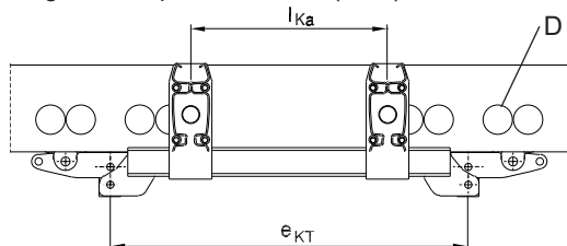
KBK II-H crane end carriage, raised, Double-girder suspension crane (ZHK)
