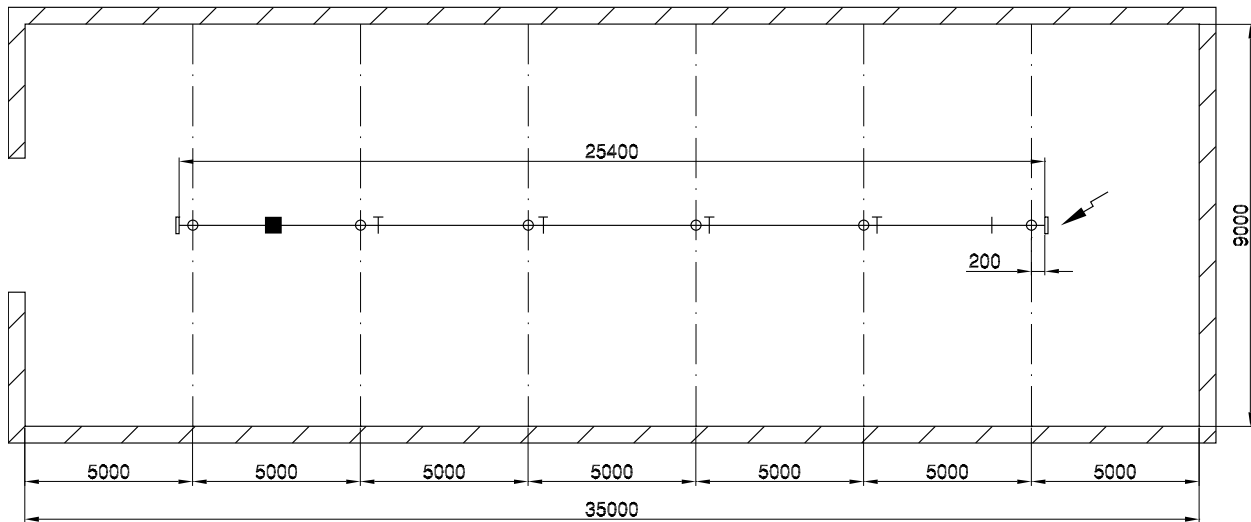
Suspension monorail
