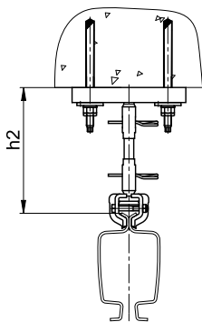
With floor fixture plate
