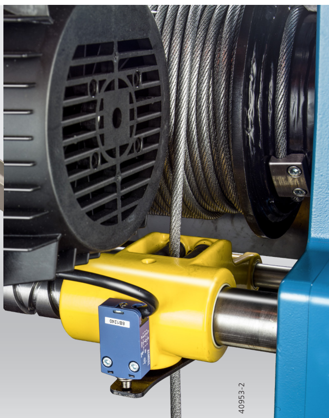
Compact design even with 180 m hook path. Multilayer technology ensures precise rope winding in up to four layers
